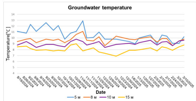
Fig. 2. Groundwater temperature
