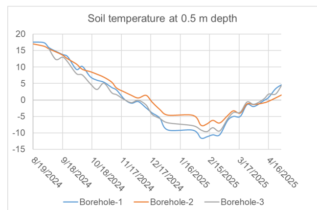
Fig. 3. Soil temperature
